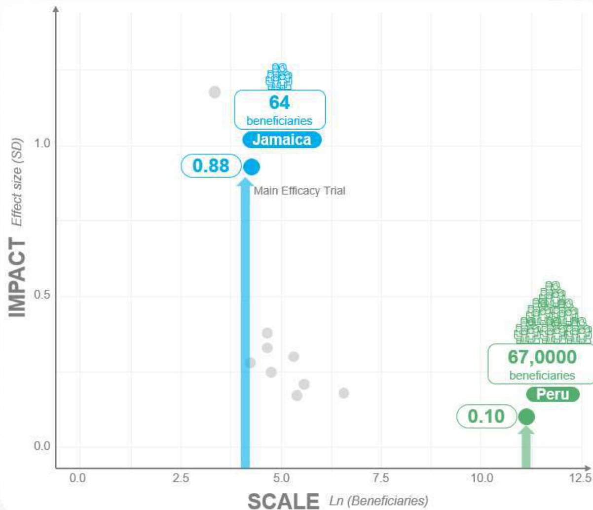
Effect Sizes of Different Replications of the Jamaican Model
